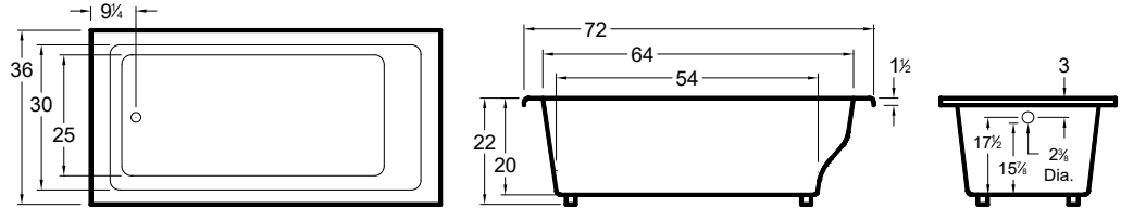
All bathtub dimensions are ± 1/2".
