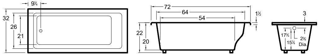
All bathtub dimensions are \pm 1/2 ".
