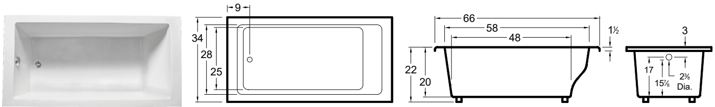
All bathtub dimensions are \pm 1/2" .
